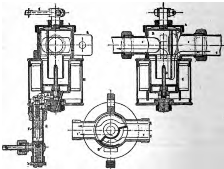
FIG. 157.—The De Dion & Bouton Vaporizer. A is the cover of the air chamber; B the air valve; C, the float; D, the mixing chamber; E gasoline supply; F, gasoline needle valve; G, valve controlling lever. Arrow (1) indicates course of air through mixing chamber; arrow (2), course of additional air through valve B.
